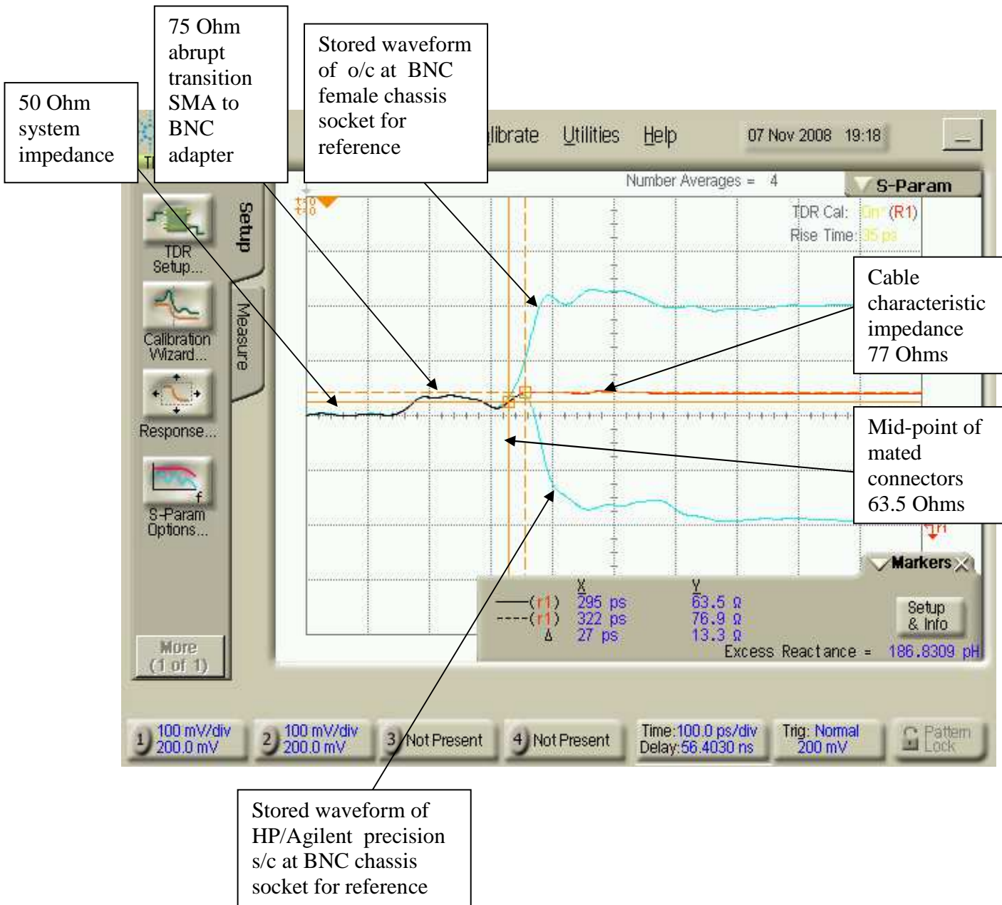
Time Domain Reflectometer (TDR) plot, with very fast pulse risetime of 35ps applied to 75 Ohm BNC plug with Belden 1505A 75 Ohm cable.
