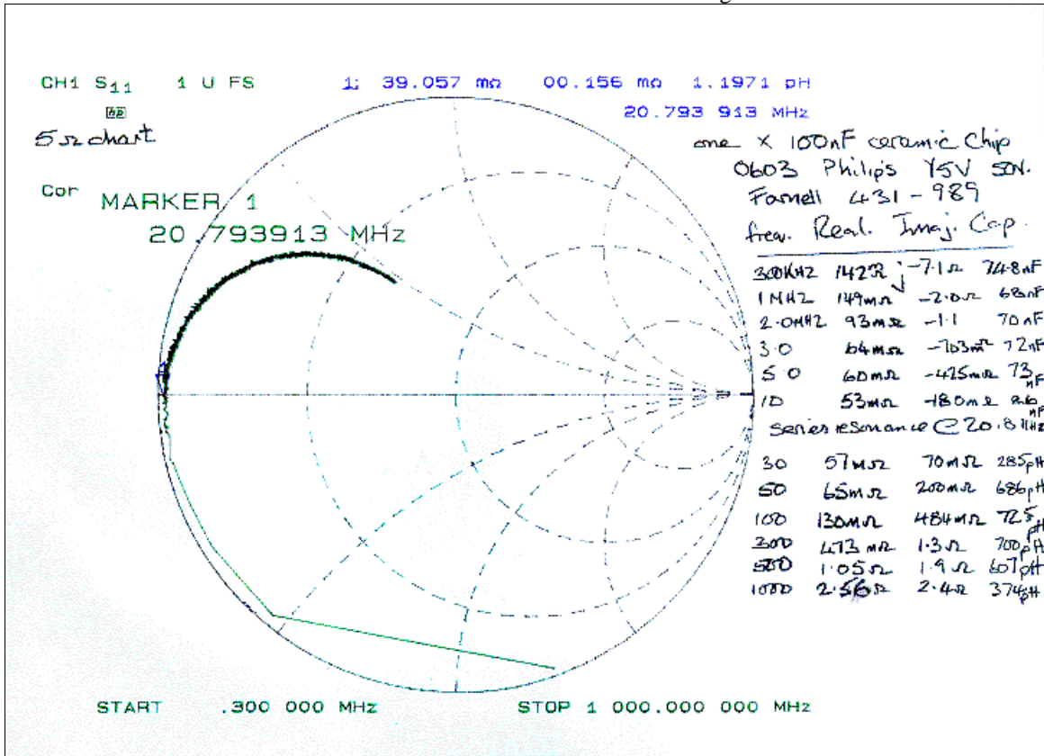
Smith Chart plot of complex reflection coefficient S 11 normalized to 5 Ohms. Component series resonance is approx. 17 - 20 MHz.
