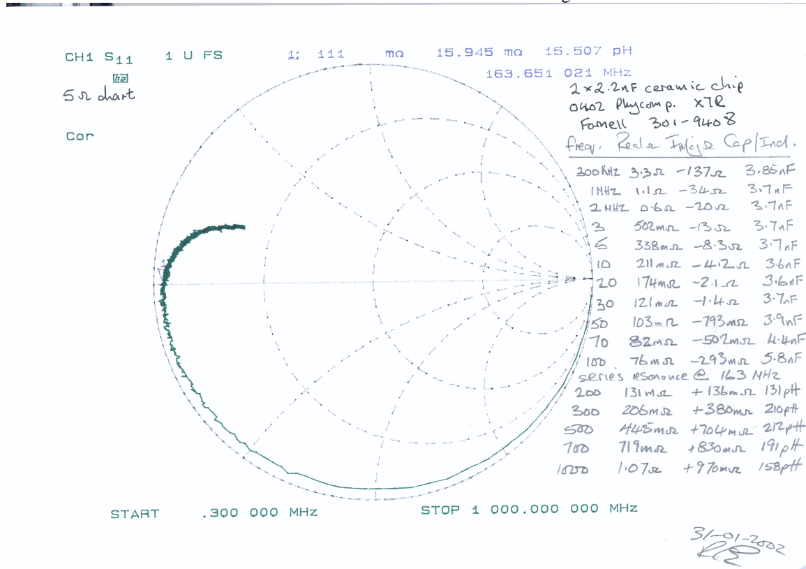
Smith Chart plot of complex reflection coefficient S 11 normalized to 5 Ohms. Component series resonance is approx. 163 MHz.
