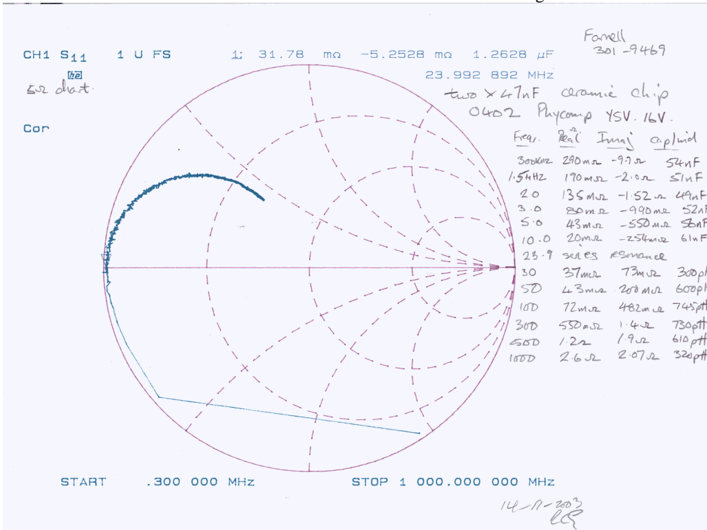
Smith Chart plot of complex reflection coefficient S 11 normalized to 5 Ohms. Component series resonance is approx. 22-24 MHz.
