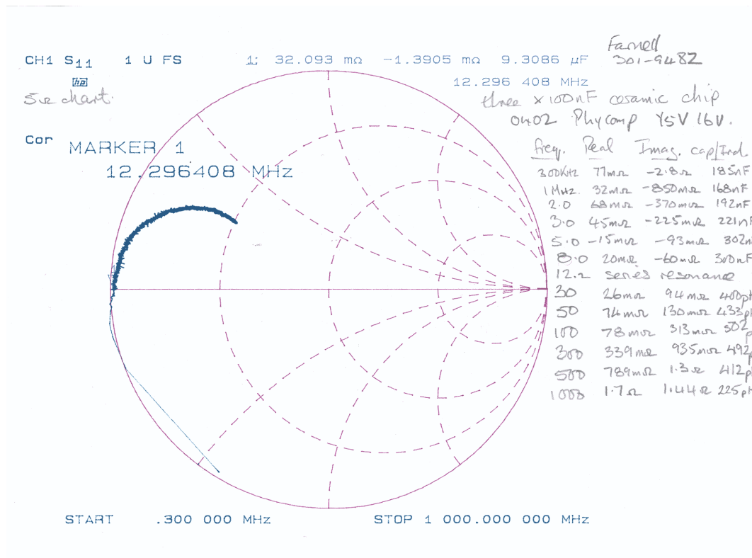
Smith Chart plot of complex reflection coefficient S_{11} normalized to 5 Ohms. Component series resonance is approx. 12 MHz.
