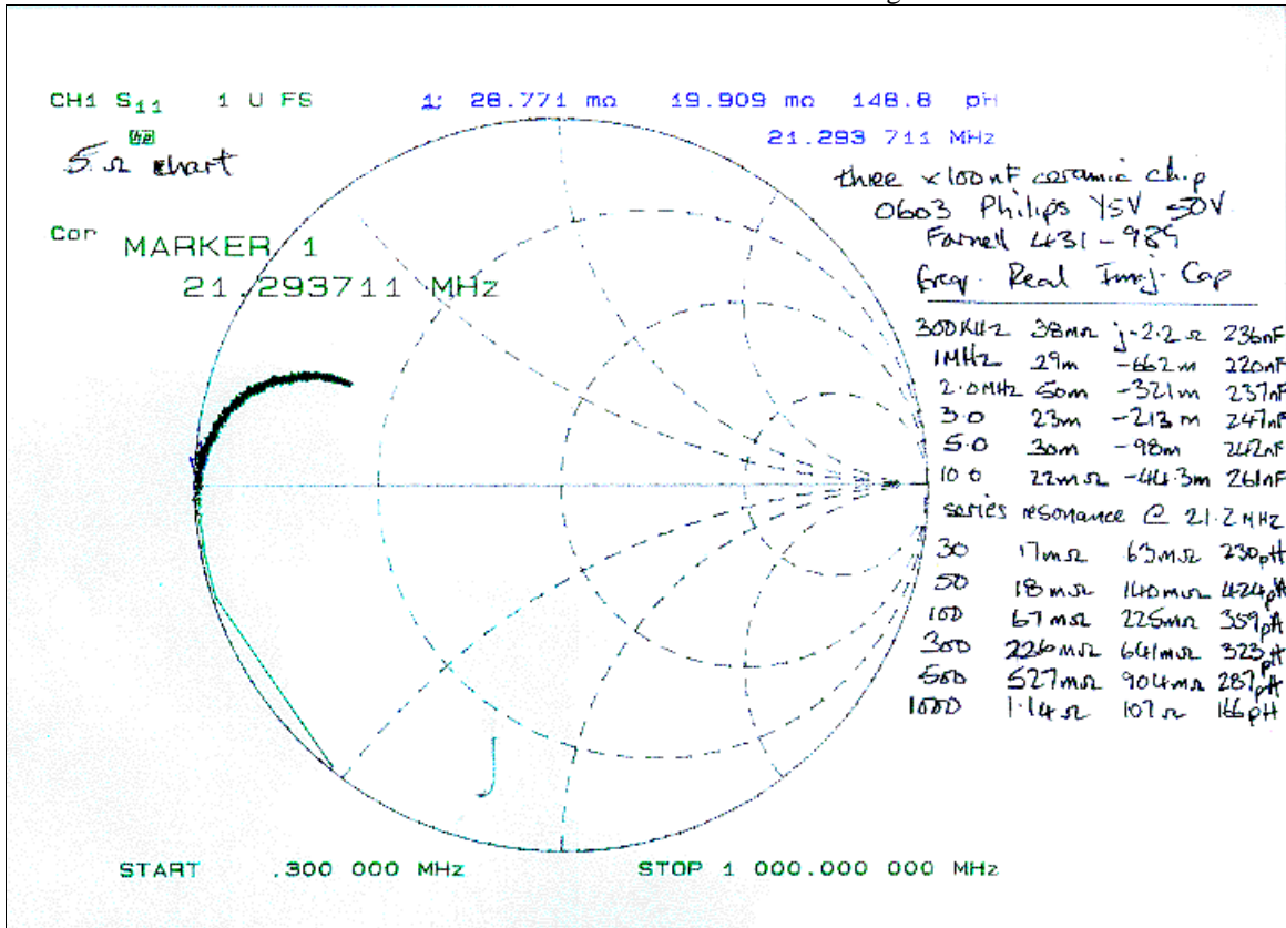
Smith Chart plot of complex reflection coefficient S 11 normalized to 5 Ohms. Component series resonance is approx. 12 - 21 MHz.
