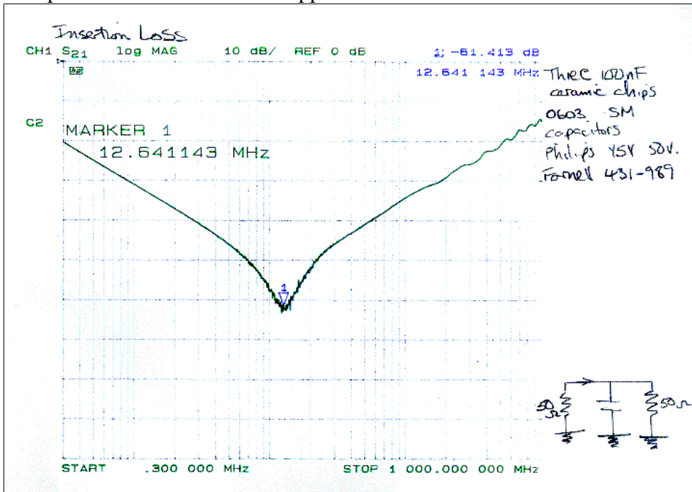
Insertion loss.
