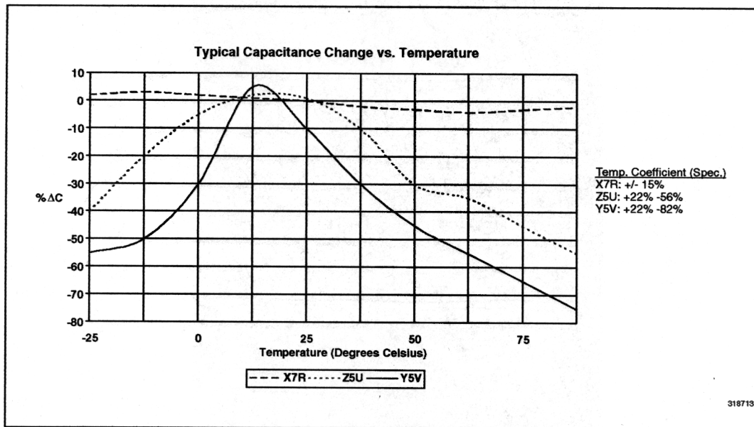
Figure 13. Typical Capacitor Characteristics
